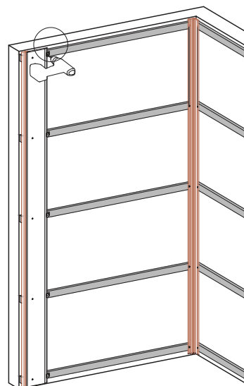
Vertical boards on horizontal battens
