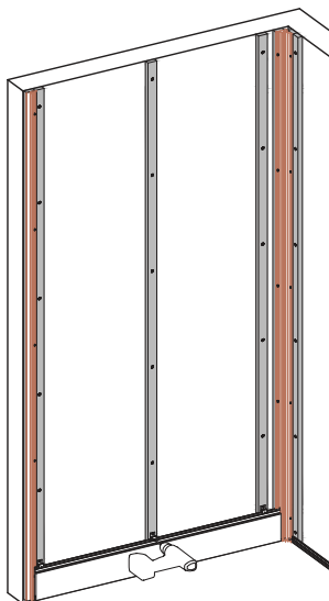
Horizontal boards on vertical battens
